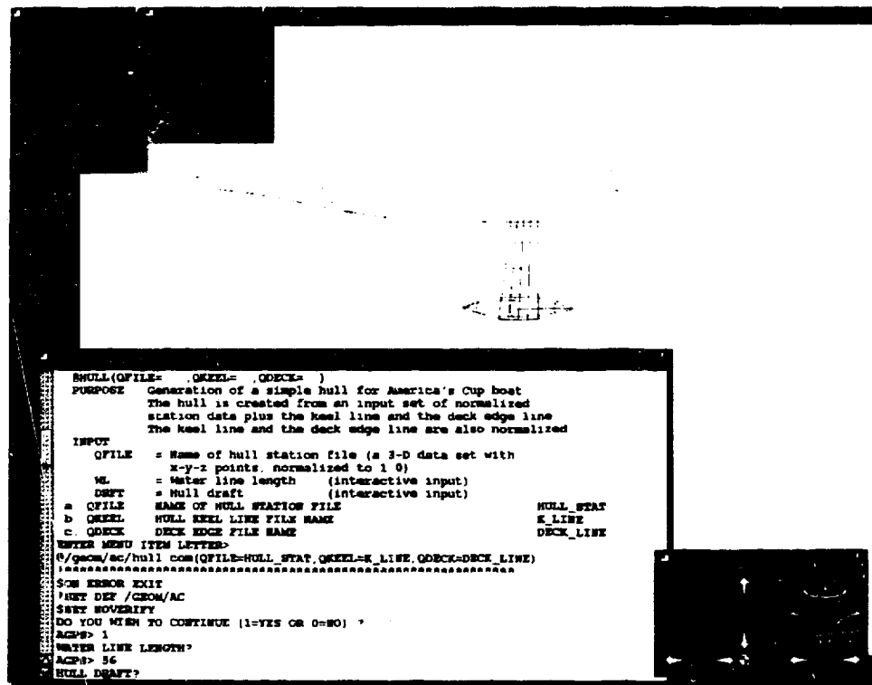
Figure 14. AGPS menu package for designing an America's Cup yacht.
