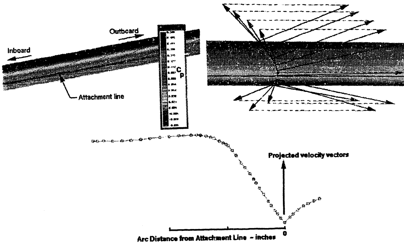
Re-theta Along Attachment Line Euler Solution (TLNS3D) glove16 + body4 Mach = 1.9 Alpha = 2.965
